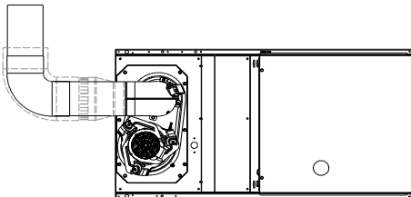
SEE NOTES: 1,2,4,7,8,9
